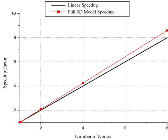
Fig. 3. Speed-up factors to 655,362 rays launched by each Tx (total of 1,310,724 launched rays )
